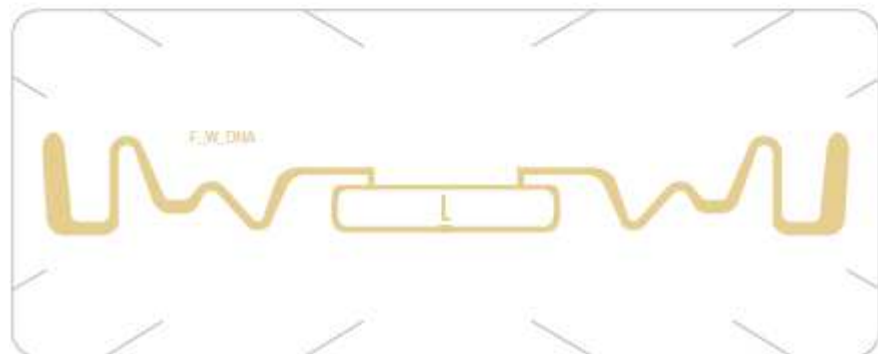
Interlayer antenna
